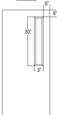
EXAMPLE: LITE METAL VISION PANEL EDGE OF DOOR TO VISIBLE LITE
