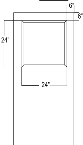
EXAMPLE: LITE WOOD BEAD EDGE OF DOOR TO CUTOUT
