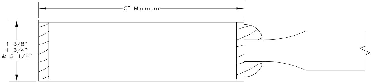
STANDARD PRESSED PANEL & STILE DETAIL
