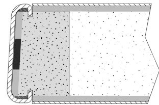
Palladium FD-5, Removable Edge
